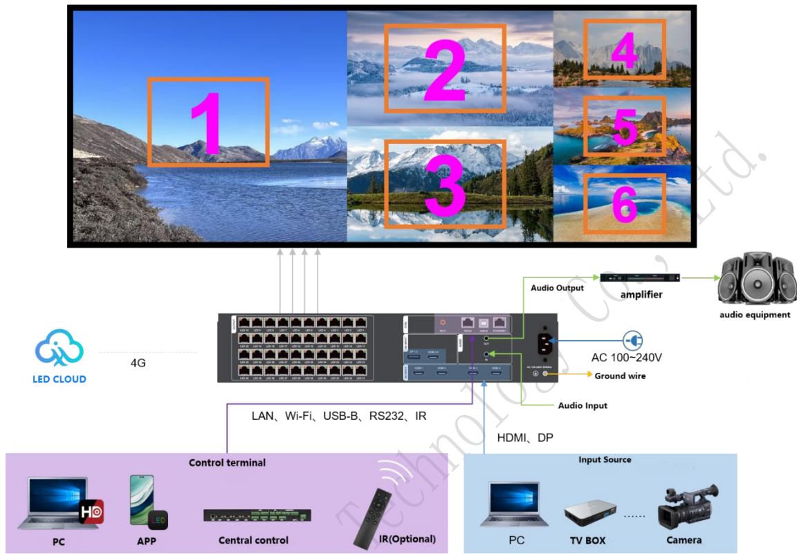
Connection Diagram
